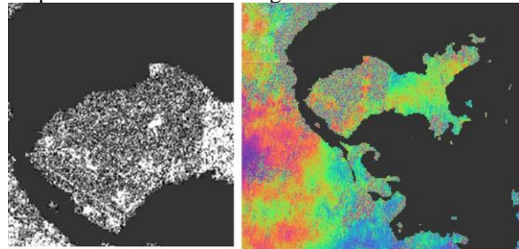
Figure 16: Coherence and phase interferogram 2015-2016
