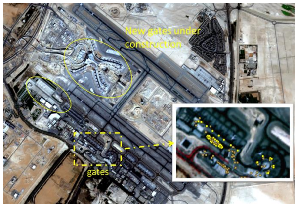
Figure 6: Abu Dhabi S2 true colour composition with OSM.
