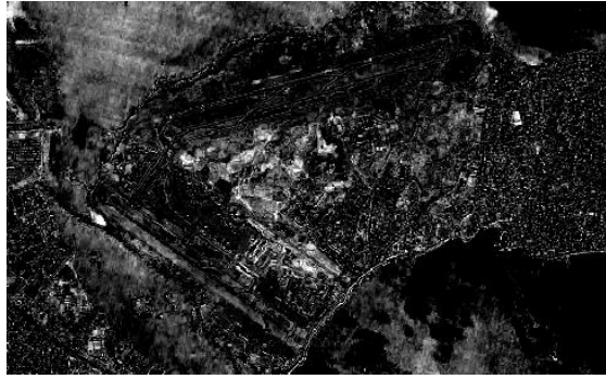
Figure 13: Change detection result with NDBI 2015-2016
